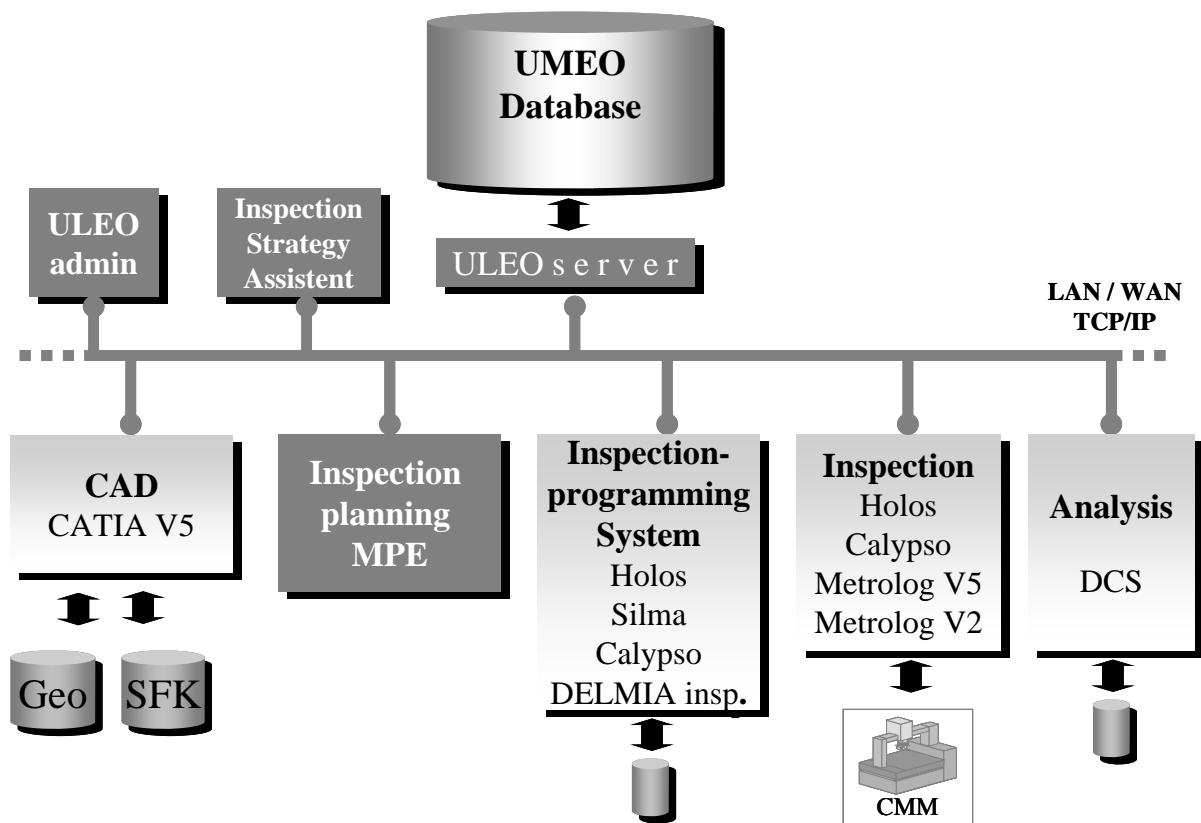
Figure 40: Inspection Scenario – Applications Involved*
