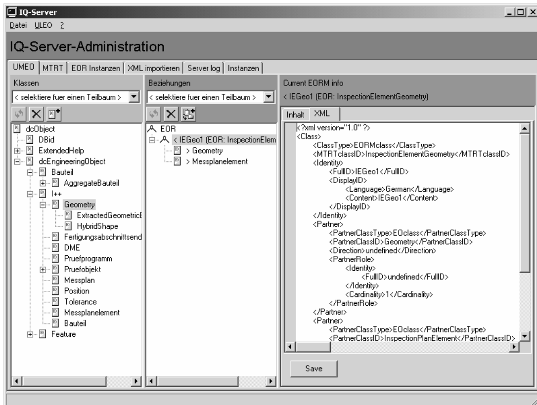
Figure 43: ULEO admin: EORM View of UMEO – XML Text Editor Tab
