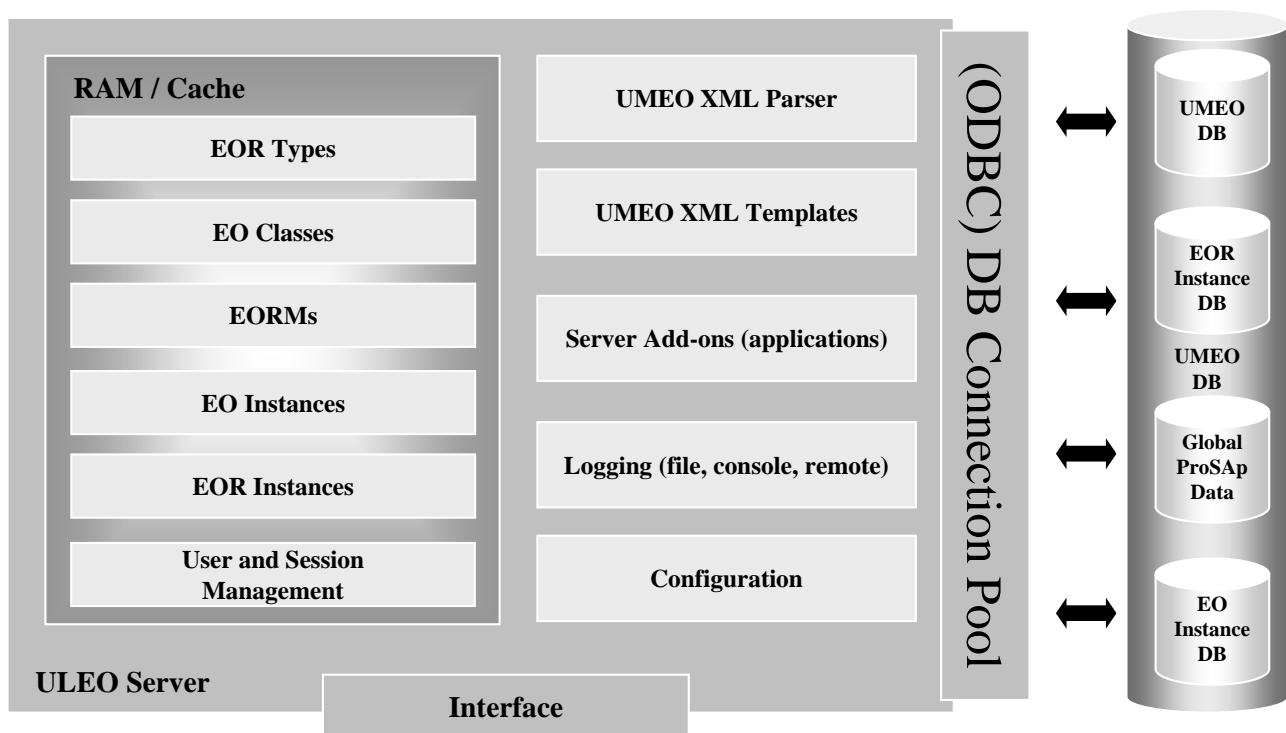
Figure 31: ULEO Server – Main Components [J. Mellens]
