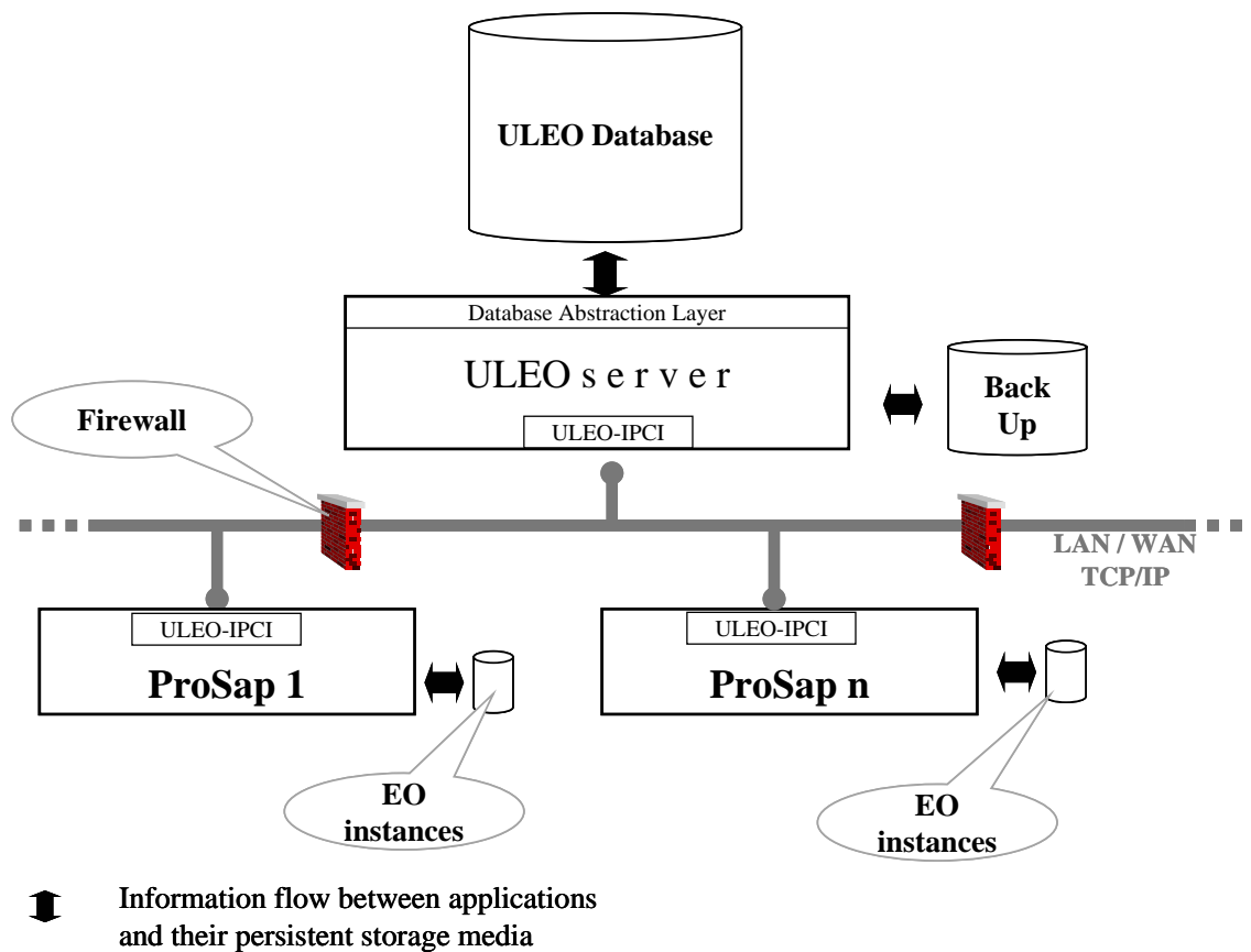
Figure 26: The Proposed Centralized ULEO Architecture
