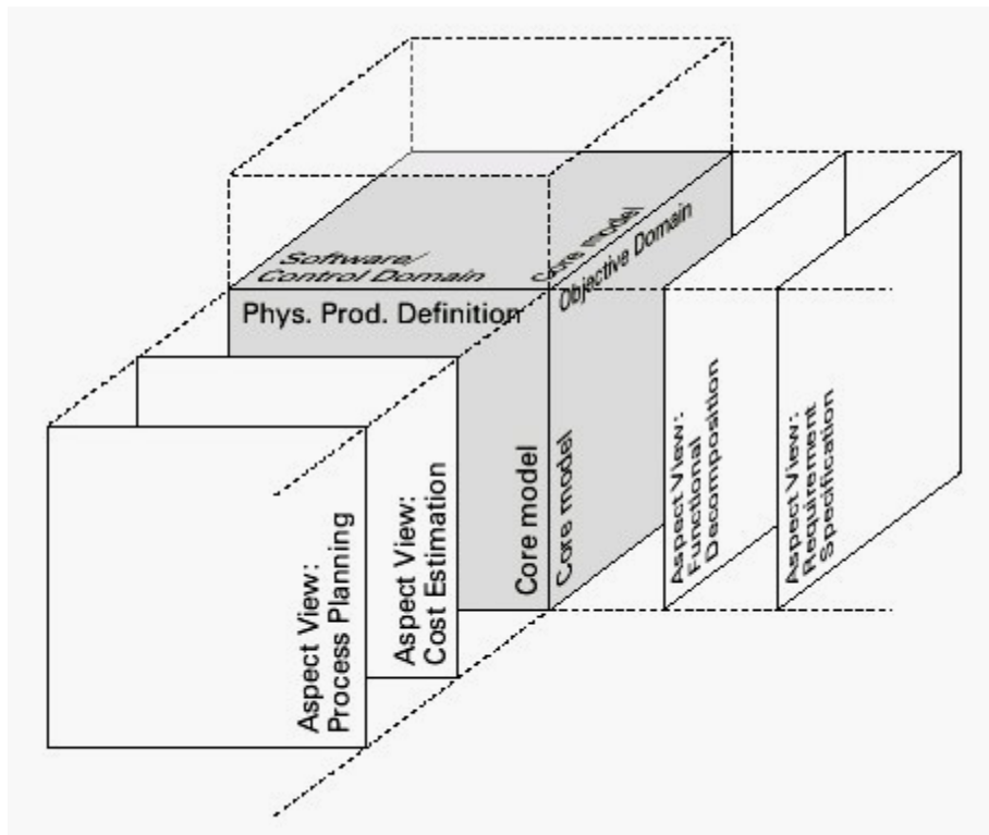
Figure 10: Basic Representation of Lutters's Product Information Structure (PRIS) [Lutters, 2001]
