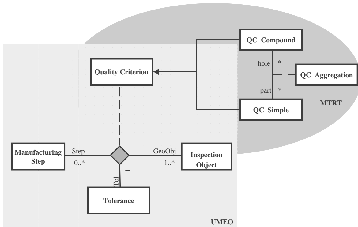
Figure 4: Impression of the I++ Information Model: The Quality Criterion Relation
