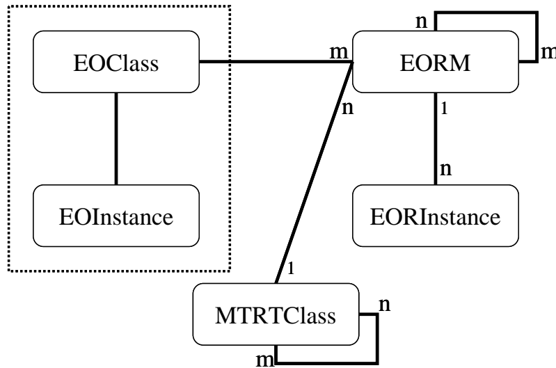
Figure 32: Simplified ER Schema of the ULEO Database [J. Mellens]
