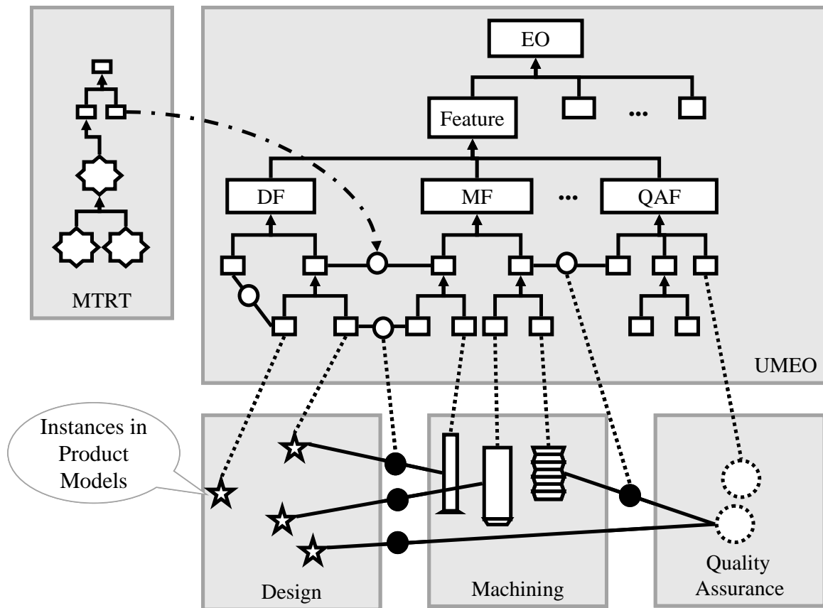
Figure 17: Partial Taxonomies in IIM/UMEO – Abstracted Illustration*
