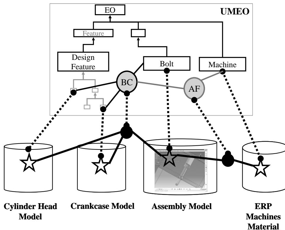
Figure 33: Assembly Feature Based on EO Constellations †
