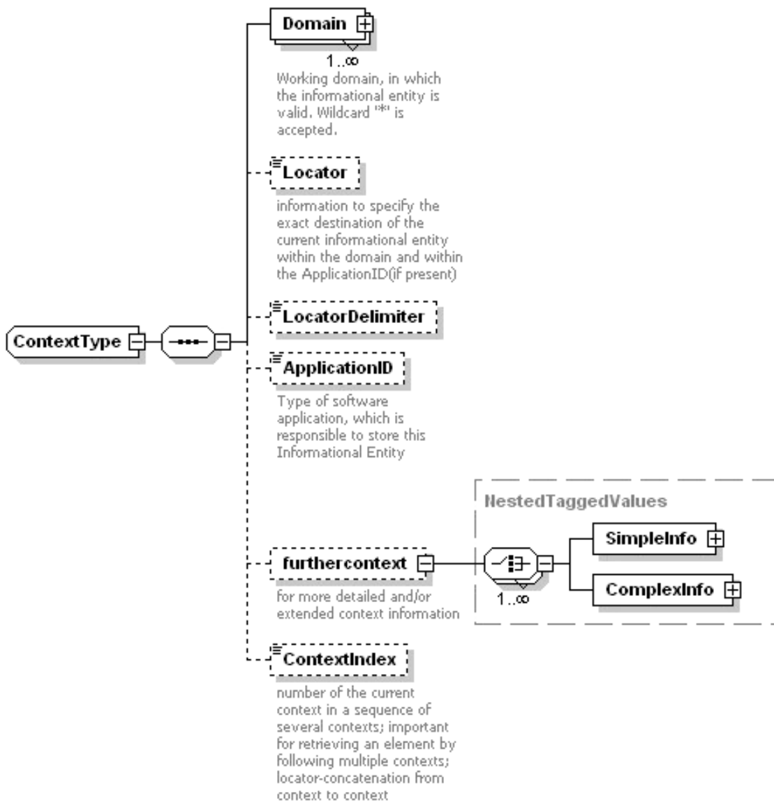
Figure 23: Context Specification in ULEO XML
