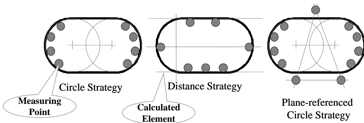
Figure 39: Various Inspection Strategies for a Slot [Th. Karthe]
