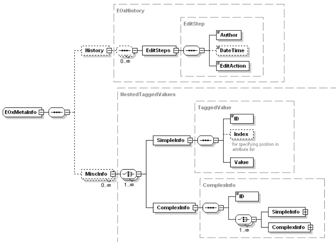
Figure 24: Universal Meta-information Schema Within ULEO XML
