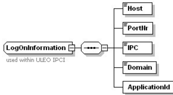
Figure 29: XML Data Type LogOnInformation within the ULEO XML Schema
