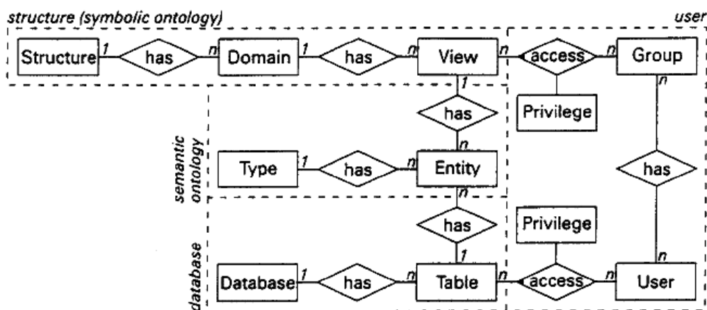
Figure 9: Arrangement of Entities in the Metabase [Lutters, 2001]
