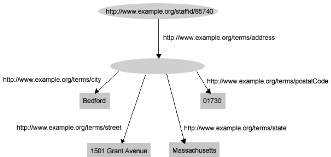
Figure 11: Blank Node for n-Ary Relations [W3C RDFprimer, 2004]
