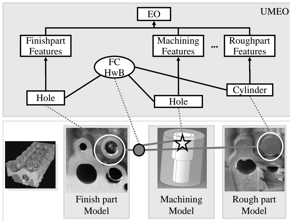
Figure 37: Feature Constellation Hole with Boss; schematic
