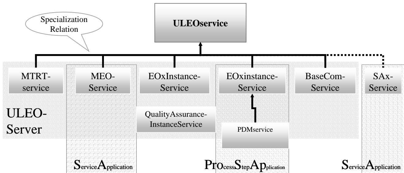
Figure 30: GIS Services and Offering Applications
