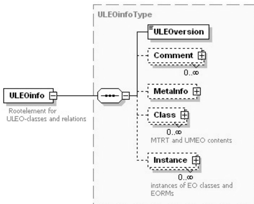
Figure 28: Uppermost Node in Most ULEO XML Blocks
