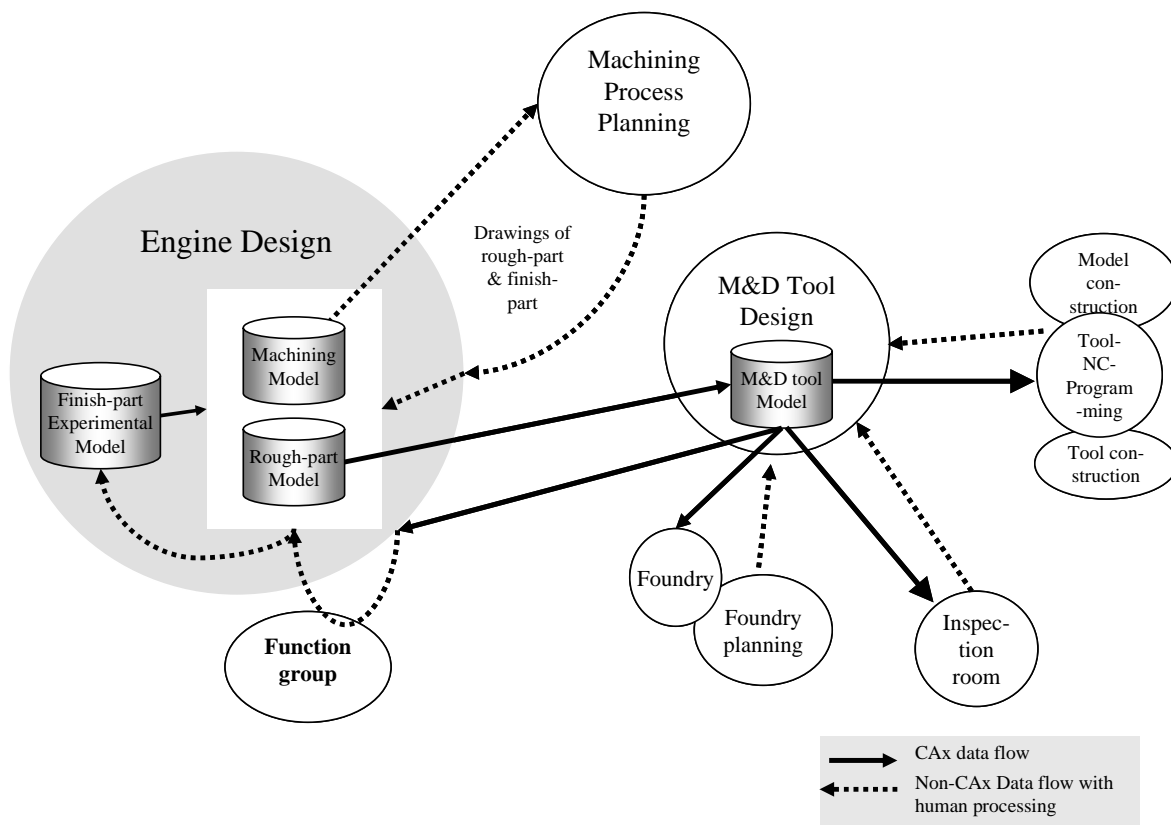
Figure 2: Cylinder Head Design in Context
