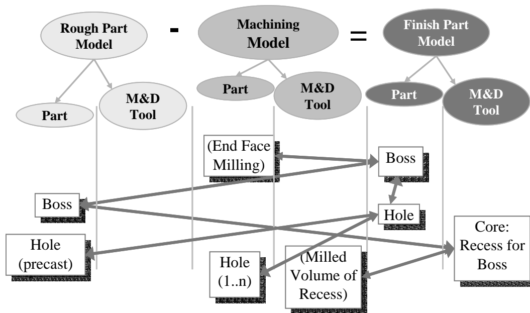
Figure 41: Hole with Boss: Relationships between EOs
