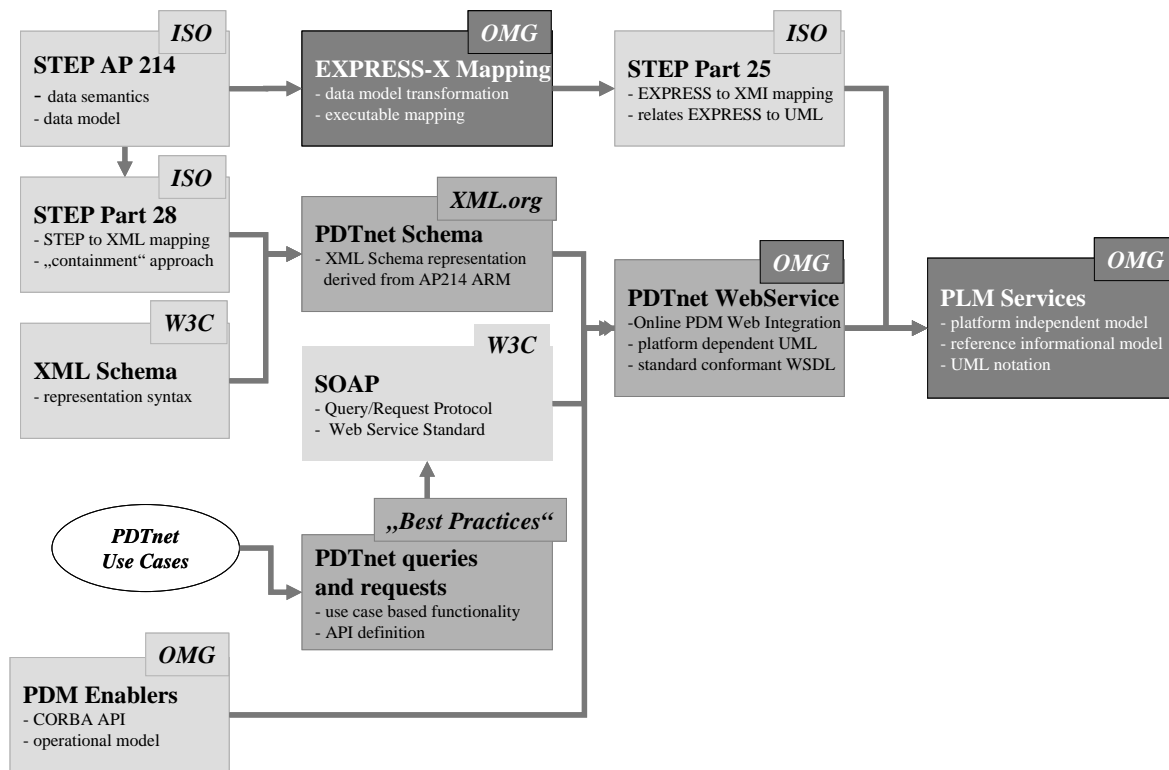
Figure 14: OMG’s PLM Services and PDTnet [PROSTEP, 2003]
