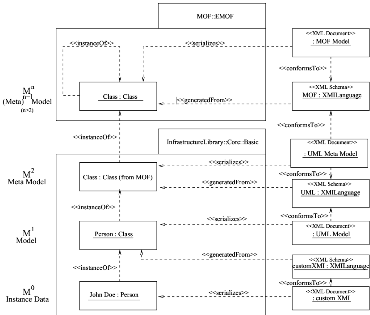
Figure 12: OMG's Four-Layer Meta-Model Architecture [Jeckle, 2004]
