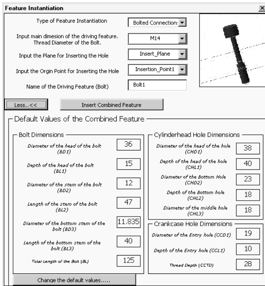
Figure 34: Instantiation Dialog for Assembly Feature EOC [Ananthanarayanan & Addala, 2002].
